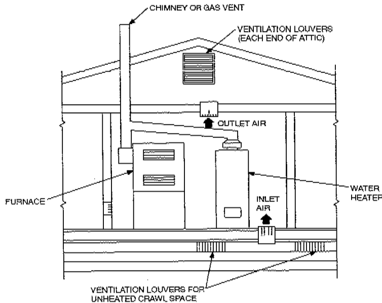
FIGURE M1703.2(4) APPLIANCES LOCATED IN CONFINED SPACES—INLET AIR TAKEN FROM VENTILATED CRAWL SPACE AND OUTLET AIR TO VENTILATED ATTIC
